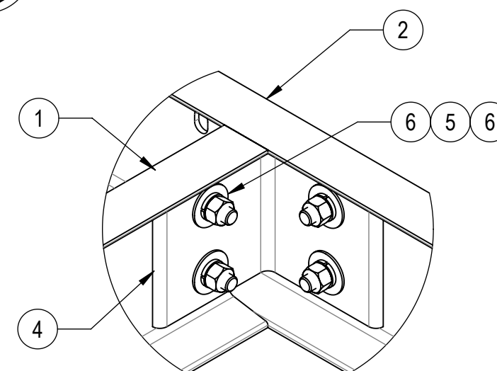
DETAIL C SCALE 1 : 5
