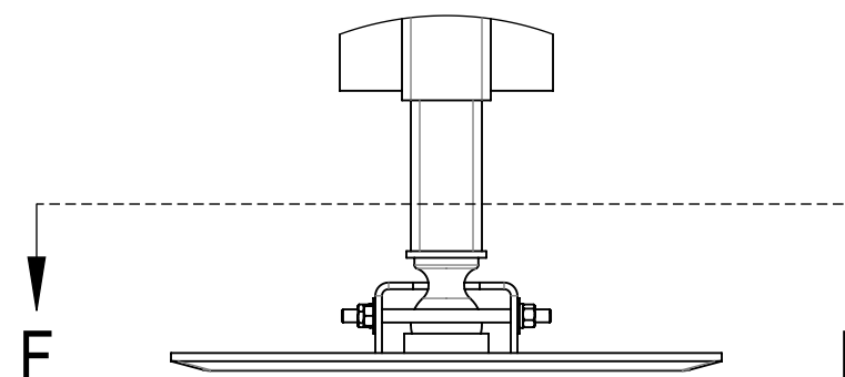
DETAIL F SCALE 1 : 6
