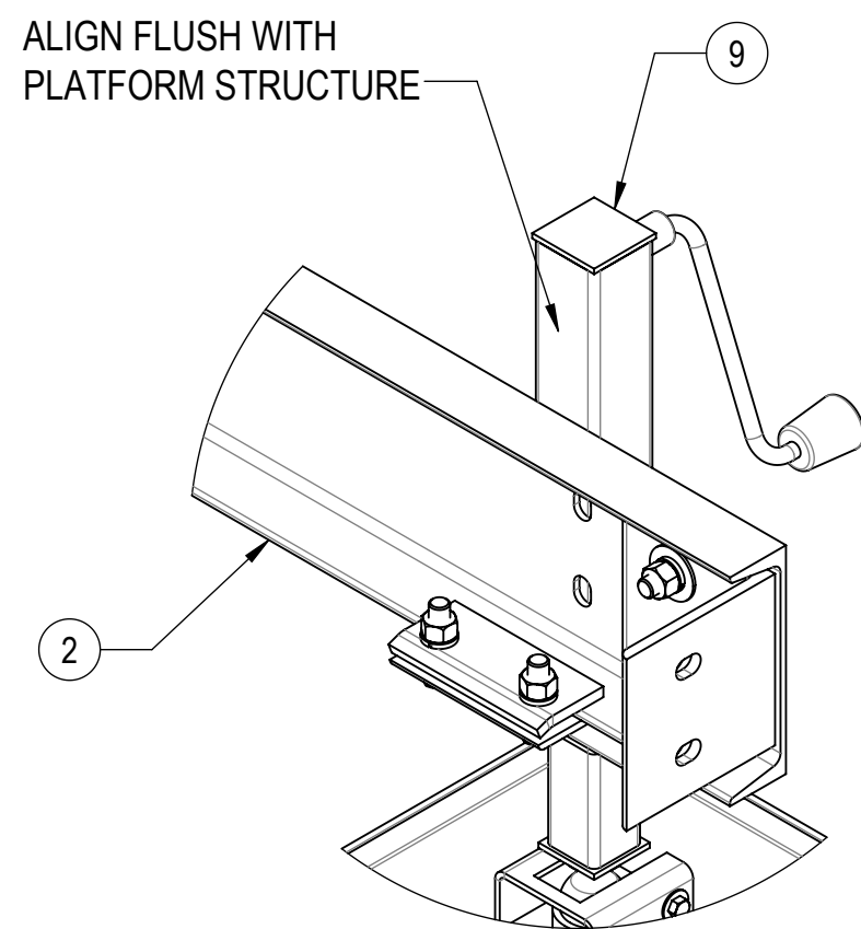
DETAIL D SCALE 1 : 6
