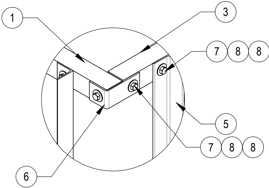
DETAIL A SCALE 1 : 8
