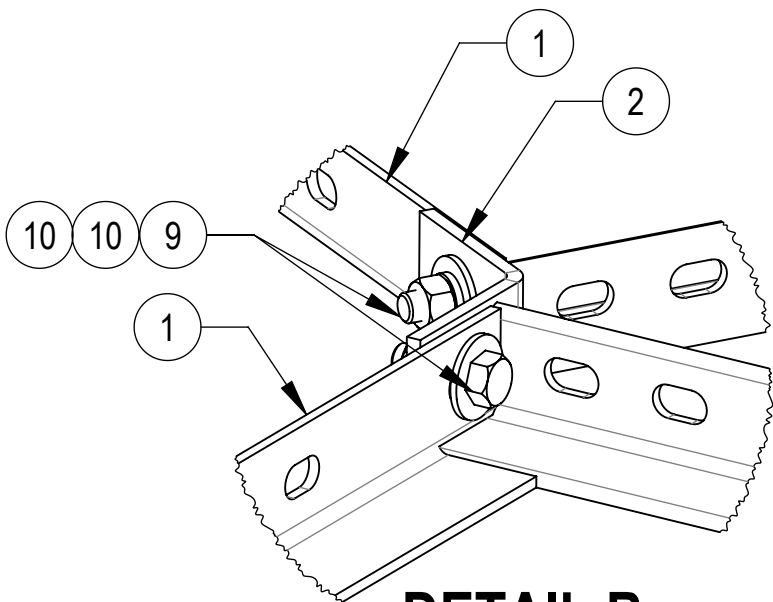
DETAIL B SCALE 1 : 3
