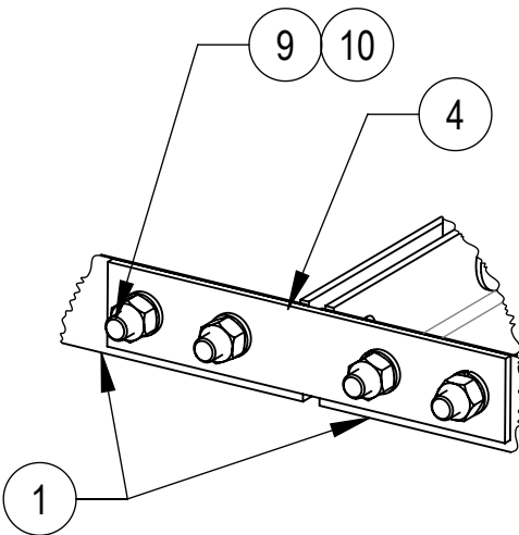
DETAIL D SCALE 1 : 4
