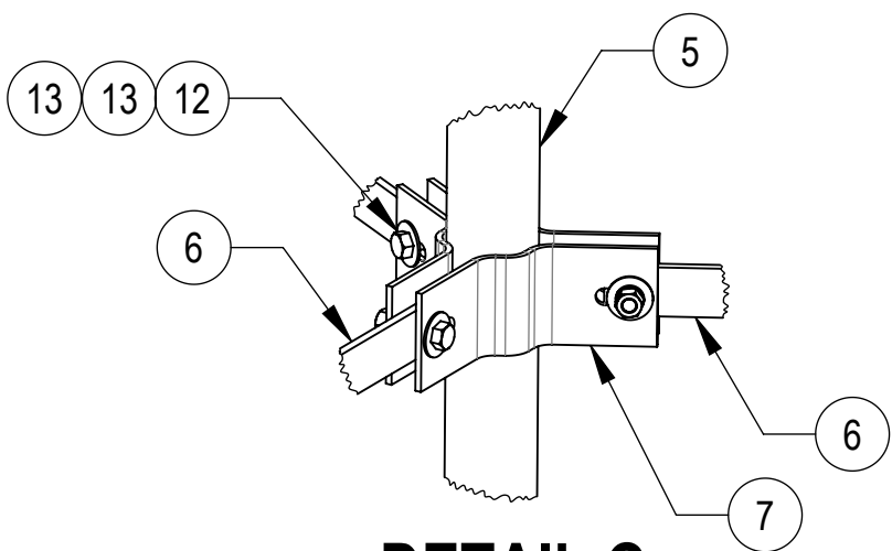
DETAIL C SCALE 1 : 8
