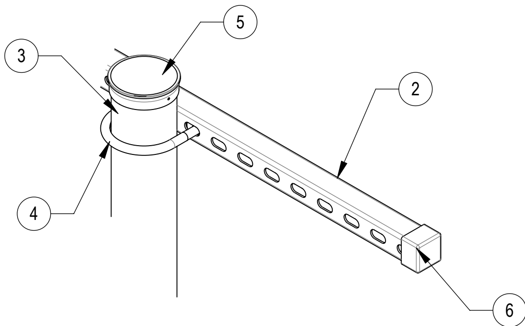
DETAIL B SCALE 1 : 5
