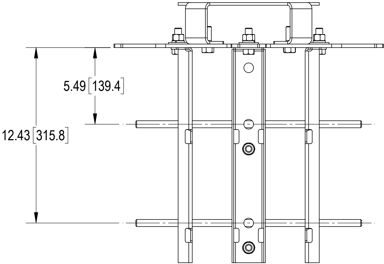
RIGHT VIEW
