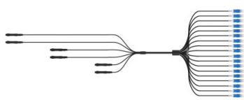
FT-36LCA9GN (18 Uniboot DLC to 6 HHC, OptiTip Compatible connector Jack 6F, SM 36 Fiber Trunk)
