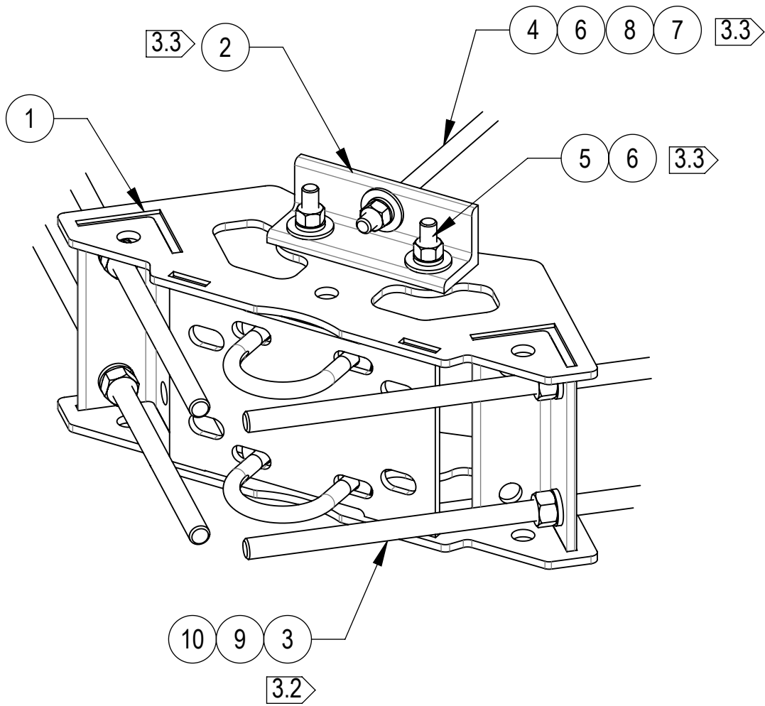
DETAIL B SCALE 1 : 4
