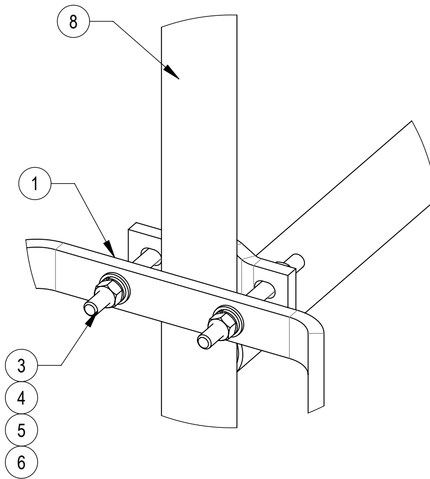
DETAIL B SCALE 1 : 3
