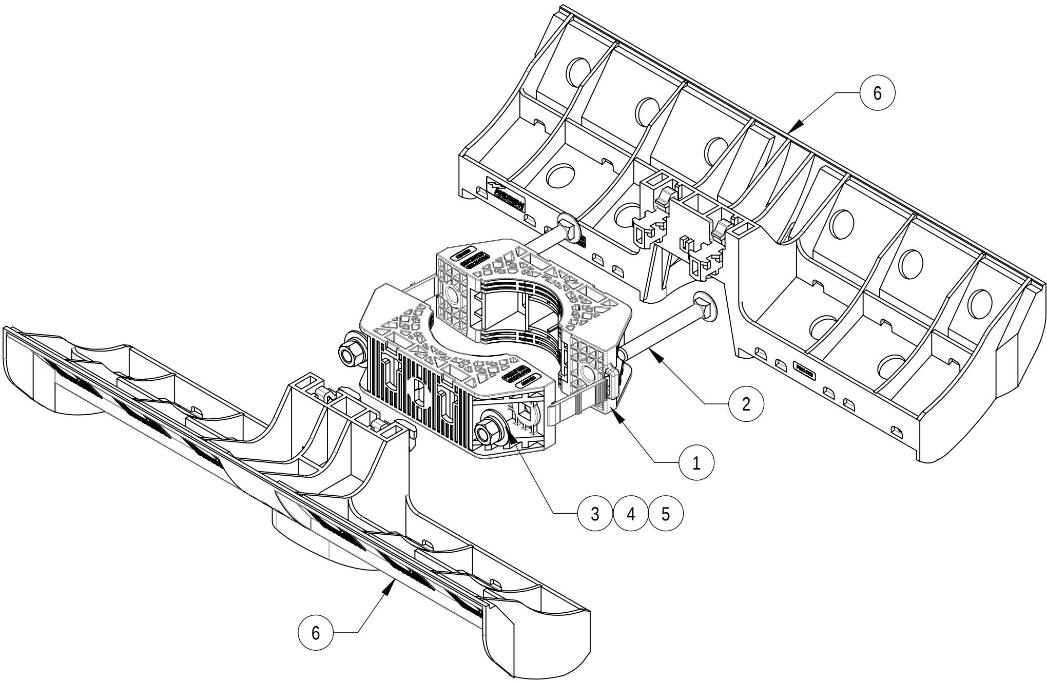
INSTALLATION ASSEMBLY
