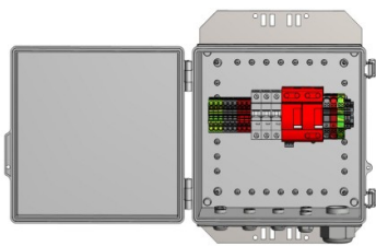
HELIAX® PTTA Enclosure with 1 SPD Class I and 3 Breakers for 3 RRU
