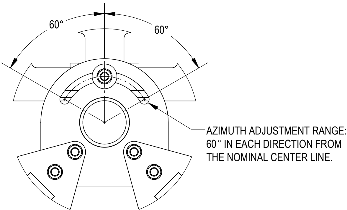
DETAIL J SCALE 1 : 4
