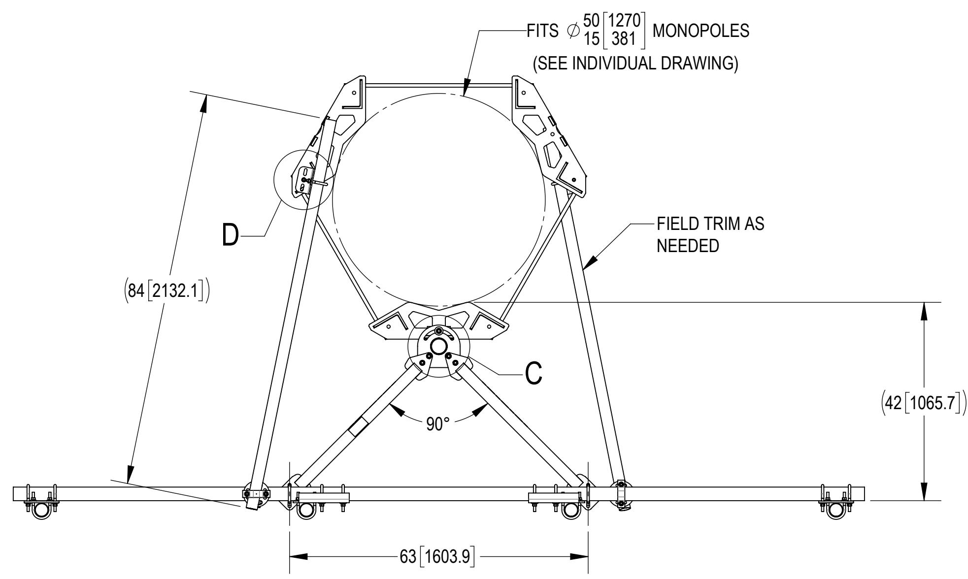
MCG22RHDX-15M12120 SHOWN FOR REFERENCE (NOT ALL CONFIGURATIONS INCLUDE ALL ITEMS SEE NOTES IN TABLE ON PAGE 3)
