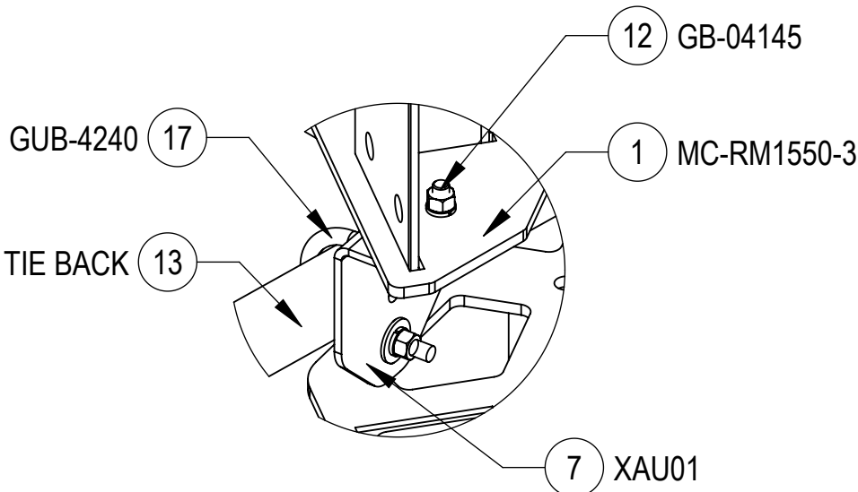
DETAIL G SCALE 1 : 5
