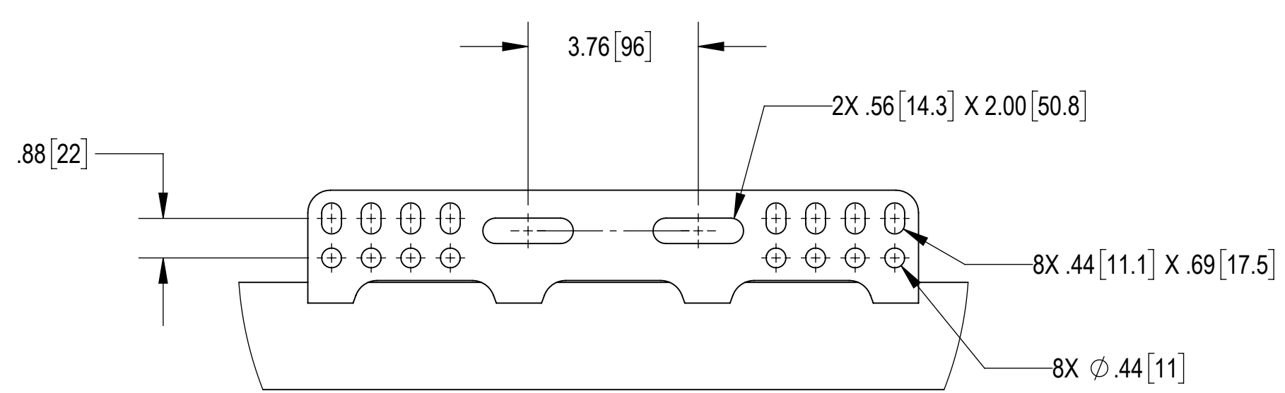
DETAIL E SCALE 1 : 3
