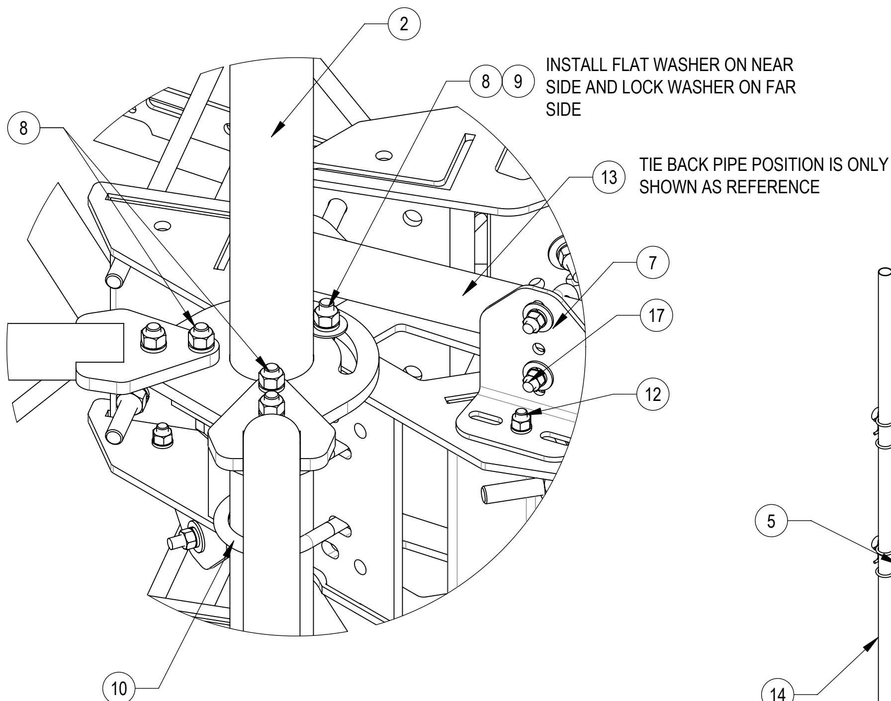
DETAIL B SCALE 1 : 4
