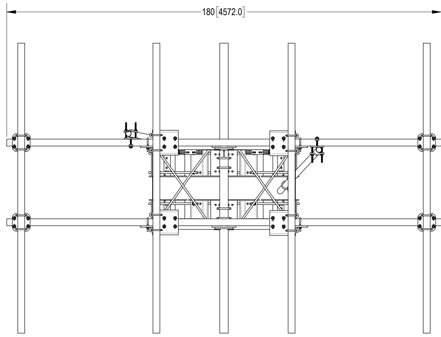
MCG22RHDX-15M12120 SHOWN FOR REFERENCE (NOT ALL CONFIGURATIONS INCLUDE ALL ITEMS SEE NOTES IN TABLE ON PAGE 3)
