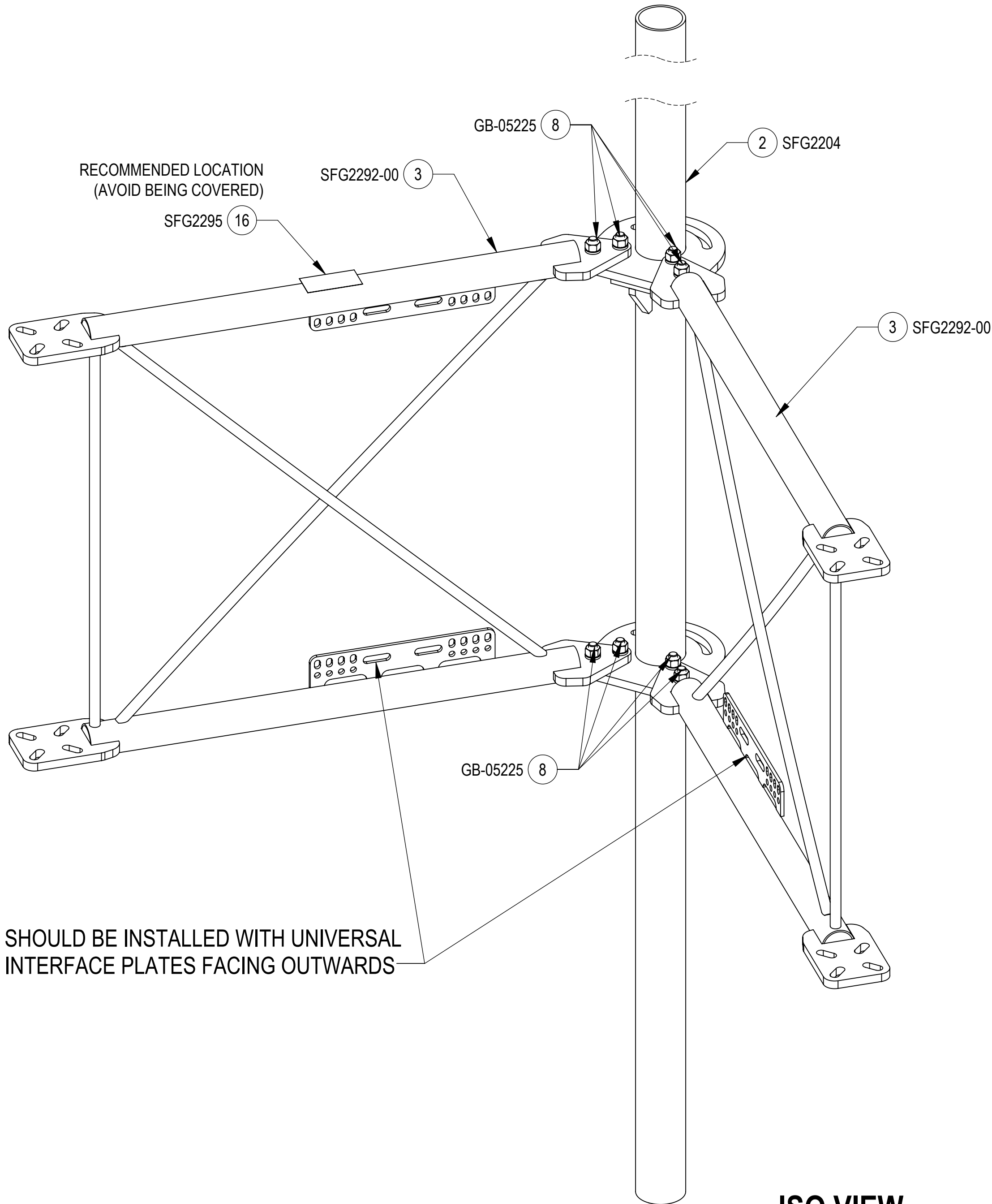
ISO VIEW
