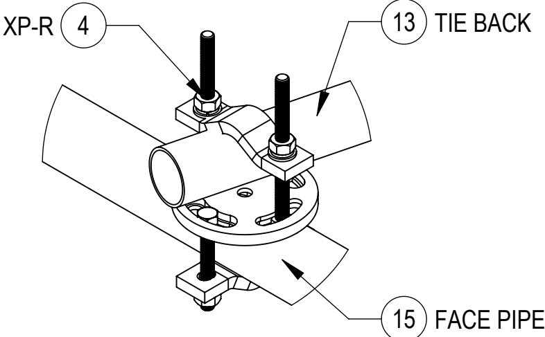
DETAIL F SCALE 1 : 5
