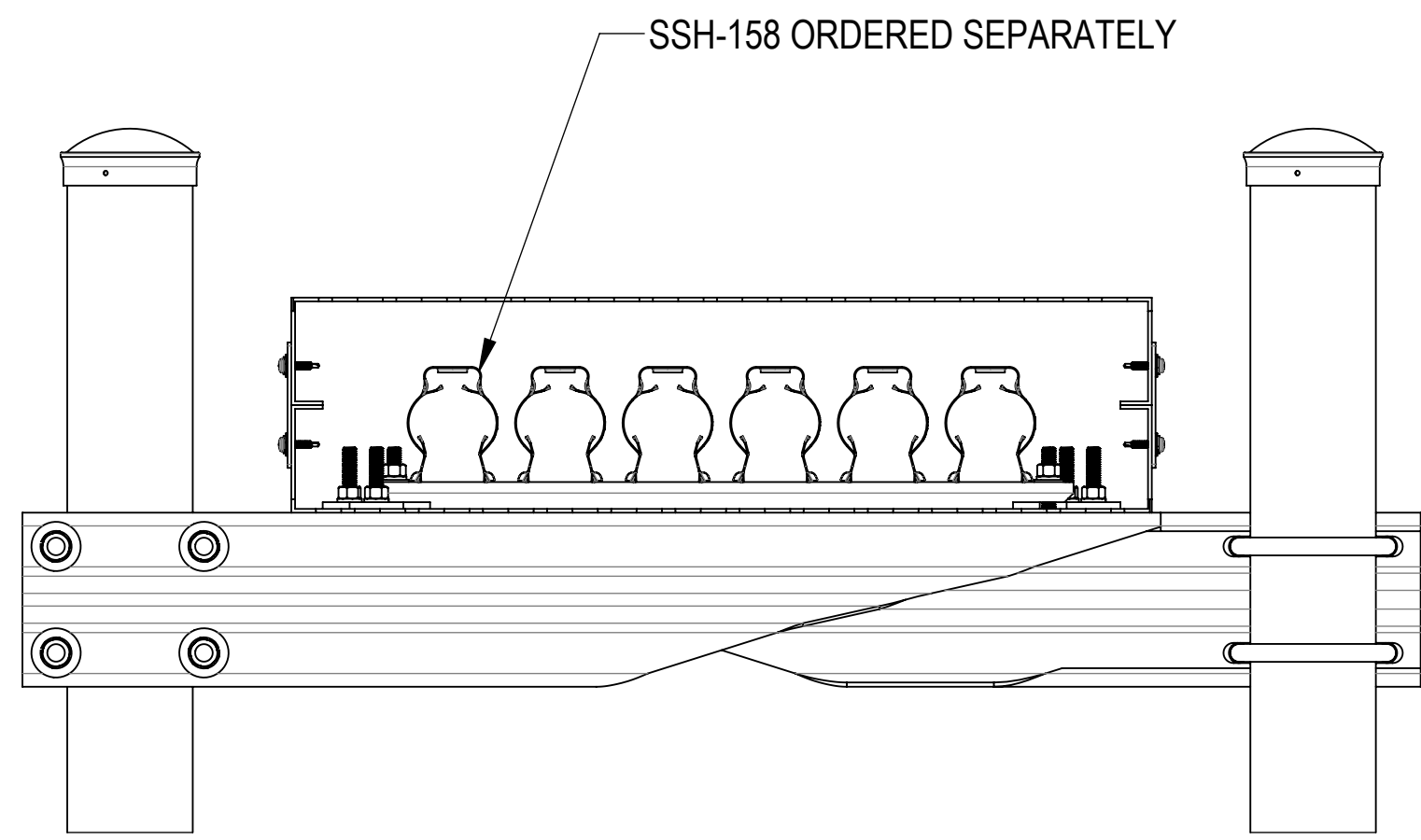
HANGER STACKED REFERENCE
