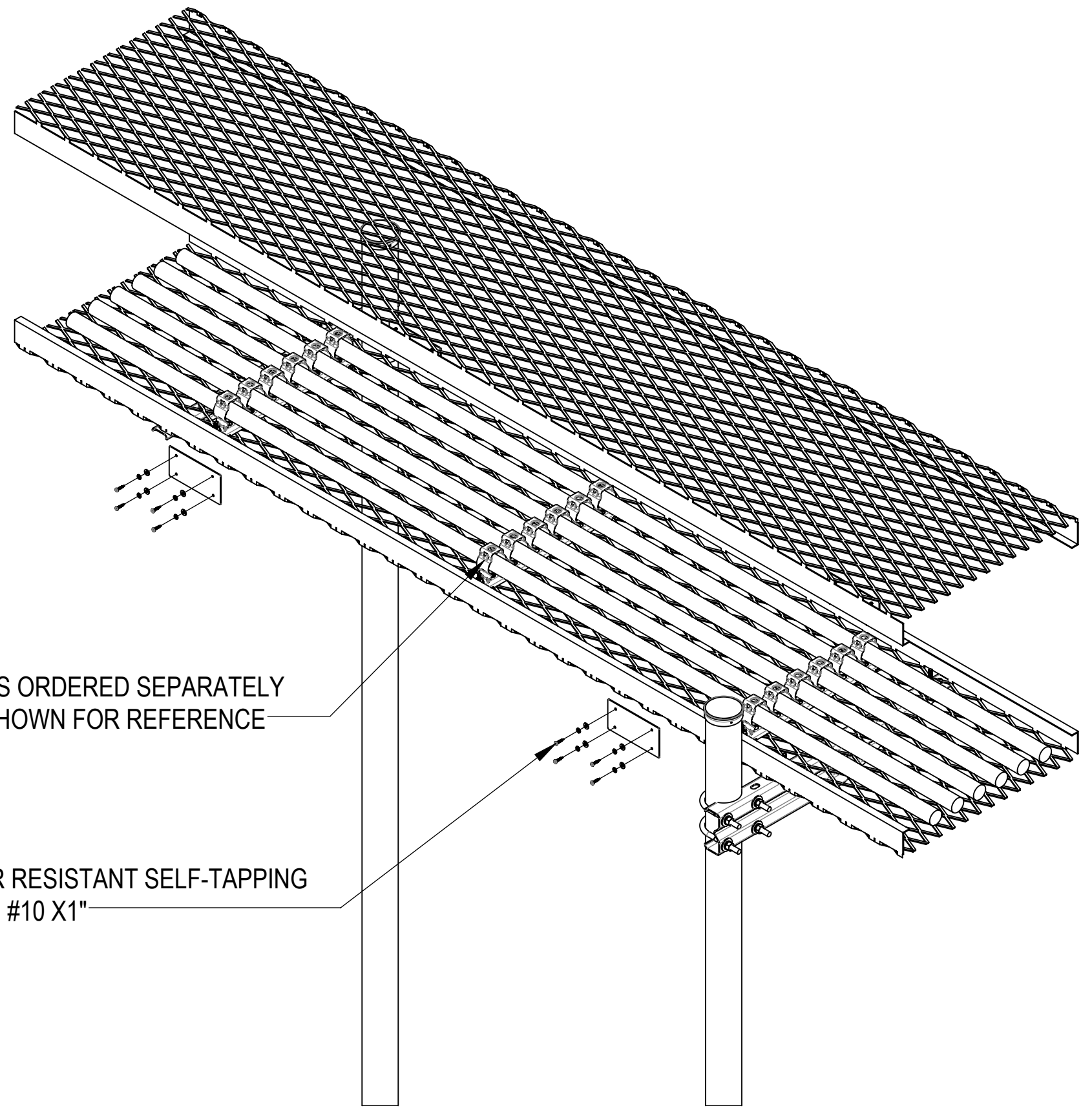
ICE BRIDGE - CABLE SECURE VIEW
