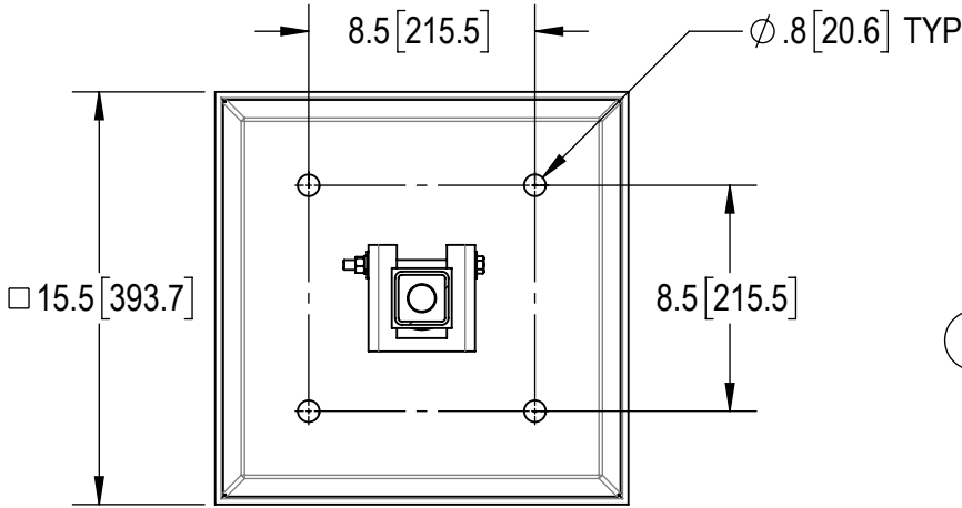
SECTION C-C SCALE 1 : 8
