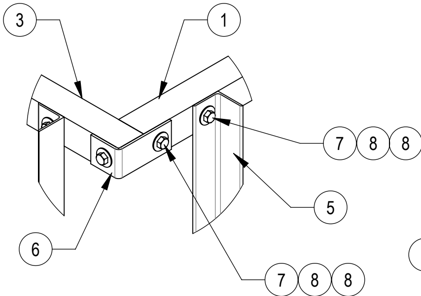
DETAIL A SCALE 1 : 8
