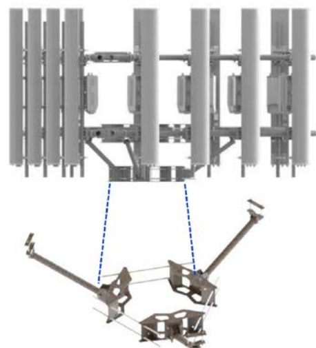
Three Sector Load Distribution Reinforcement Kit RK-36-3S
