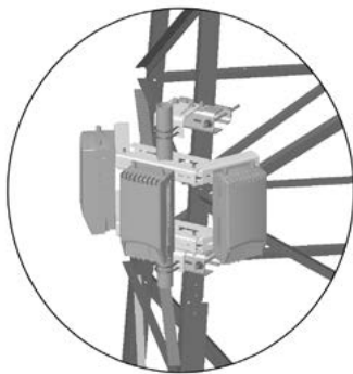
Universal Sliding Pipe Mount PM-SU35-48
