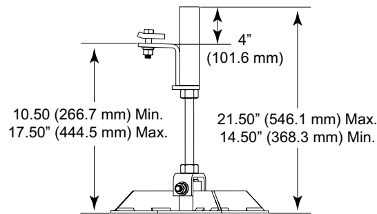
Weight Dispersement Legs EQ-P-DF
