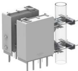
RRU Mount, Ericsson (RR-FA4)
