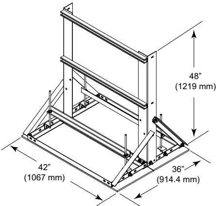
Non-penetrating Roof-top Mounting RRU's RR-TFS
