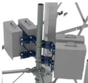
APEX Radio Mount (RR-APEX4)
