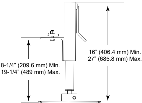
Adjustable Legs EQ-P-AL
