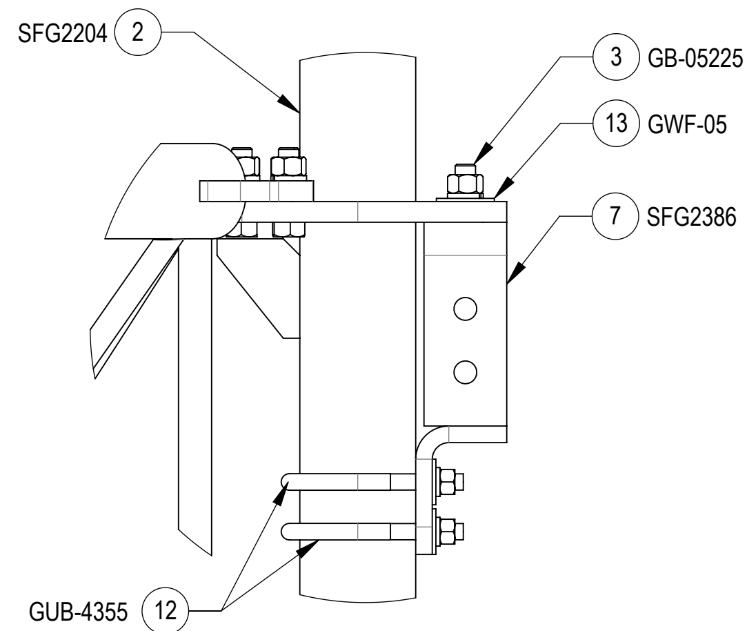
DETAIL H SCALE 1 : 4
