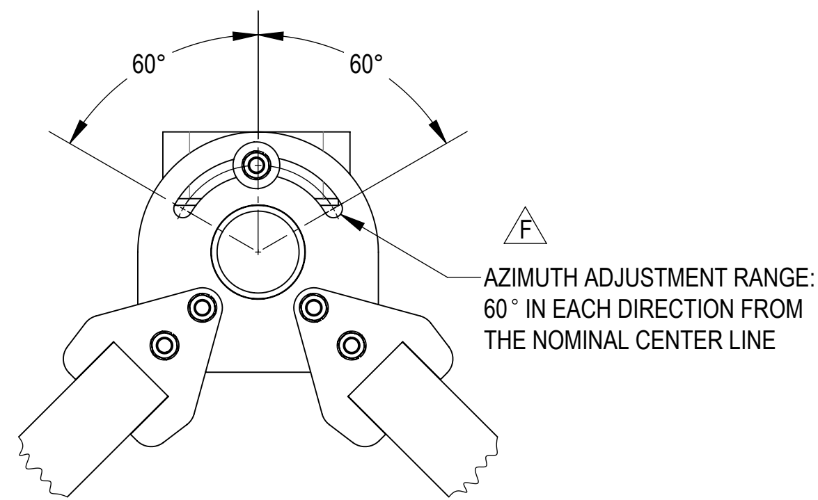
TOP CROP VIEW
