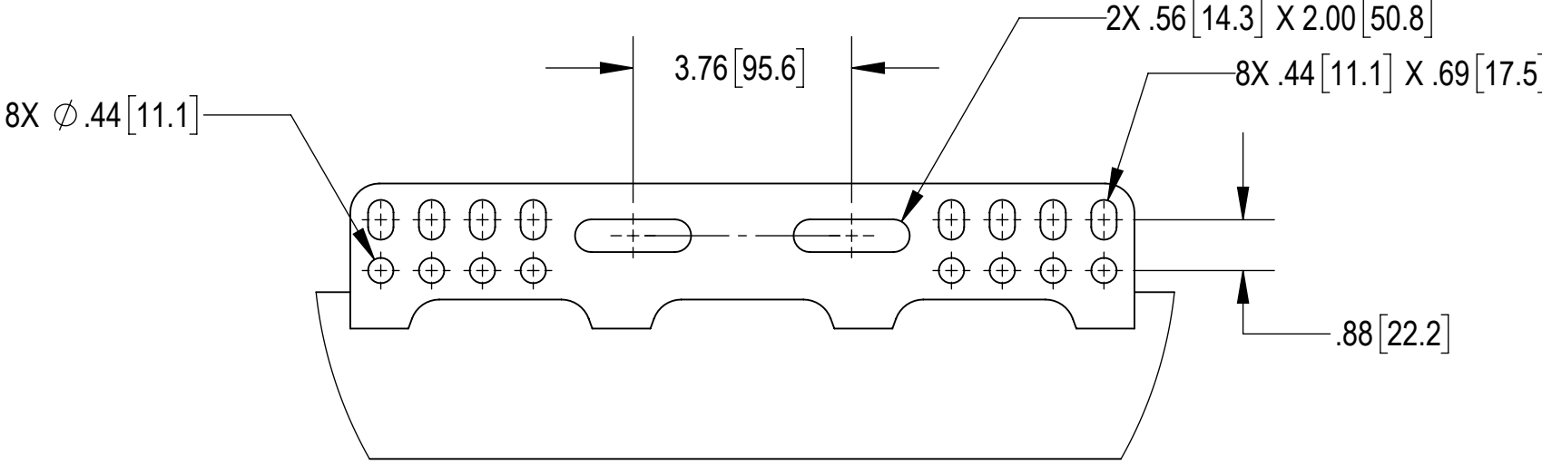
DETAIL F SCALE 1 : 3
