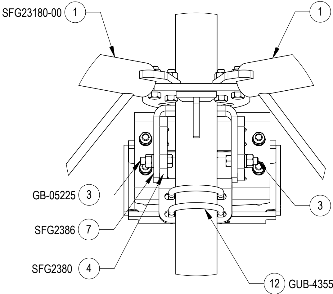
DETAIL ISO TOP ROTATED VIEW SCALE 1 : 5
